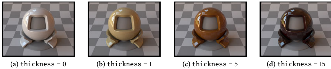
Figure 14: The effect of the layer thickness parameter on a tinted coating ( \sigma_T = (0.1, 0.2, 0.5) )
